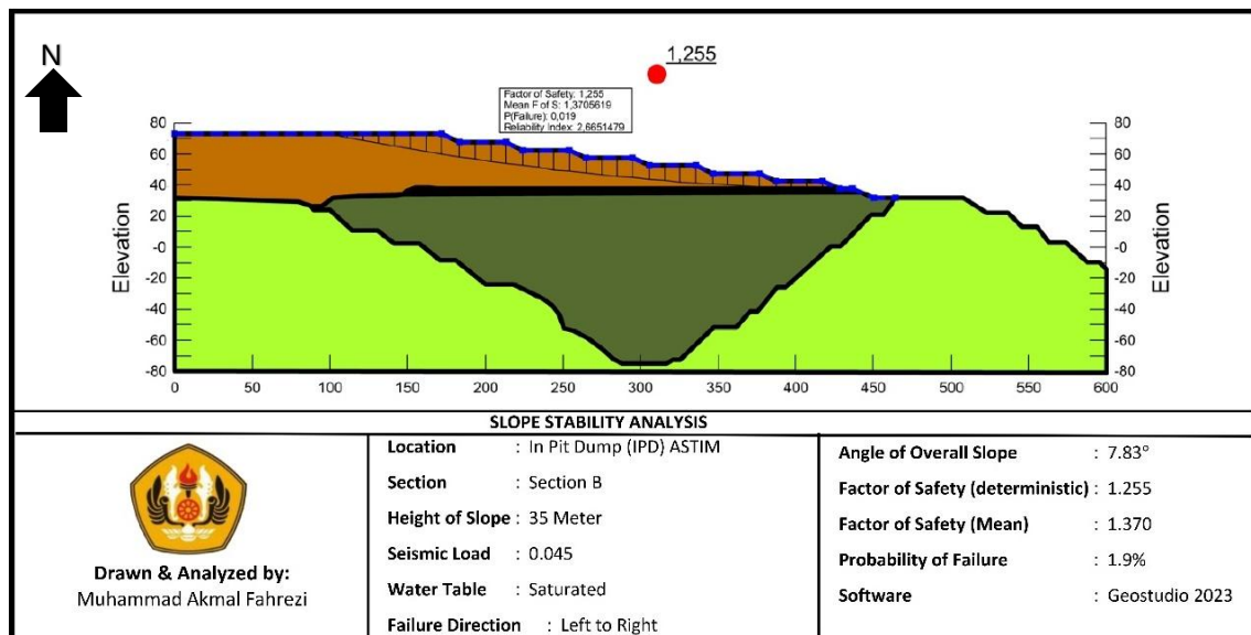
Figure 12. Slope stability analysis result design recommendation in dynamic condition
