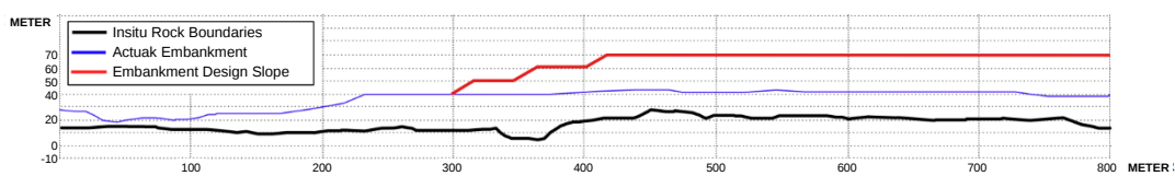
Figure 5. Design of embankment Slope A – A'
